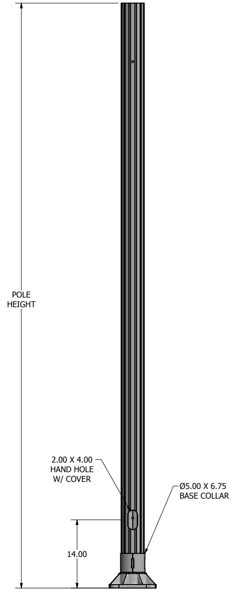
POLE DETAIL
