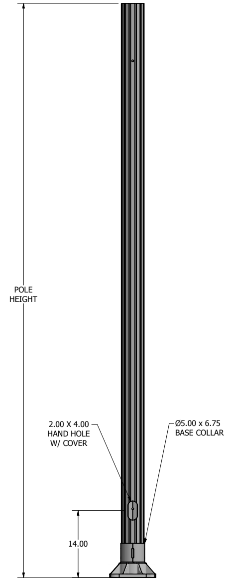
POLE DETAIL
